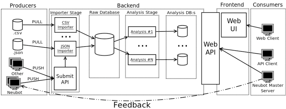
Figure 1: NeuViz architecture
